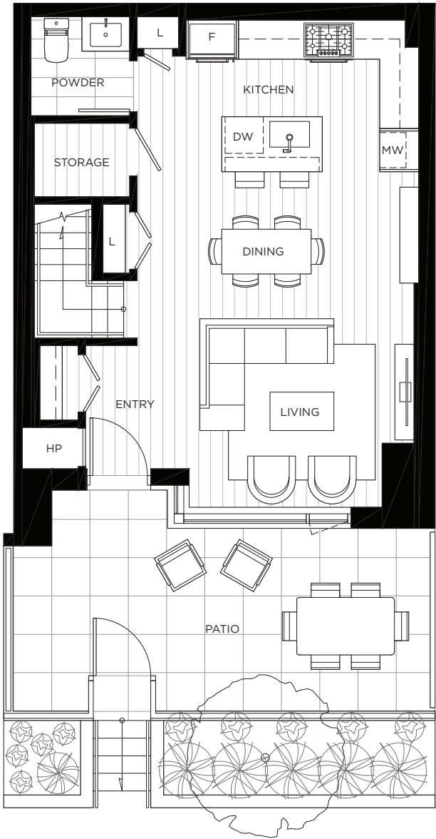
MAIN LEVEL
